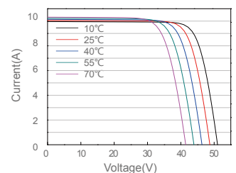
Current-Voltage Curve JAM72S01-380/PR
